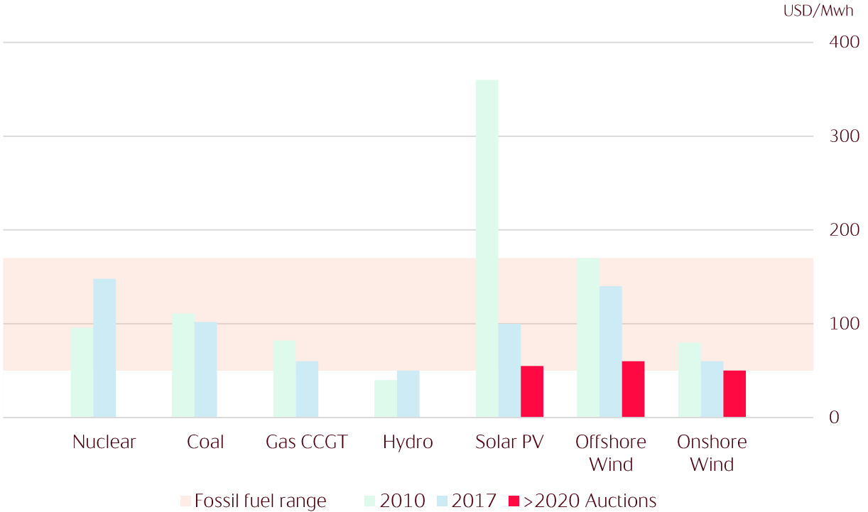
Global levelised cost of electricity from utility-scale generation technologies
